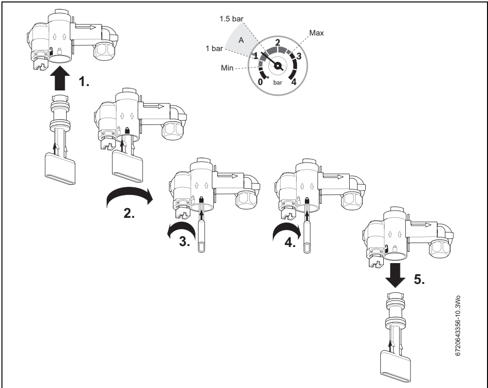
Fig. 3 Keyed filling link
